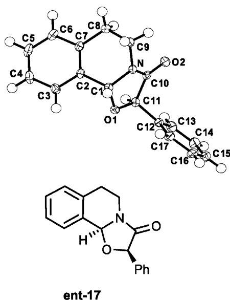
Figure 4. X-ray crystal analysis of ent-17
